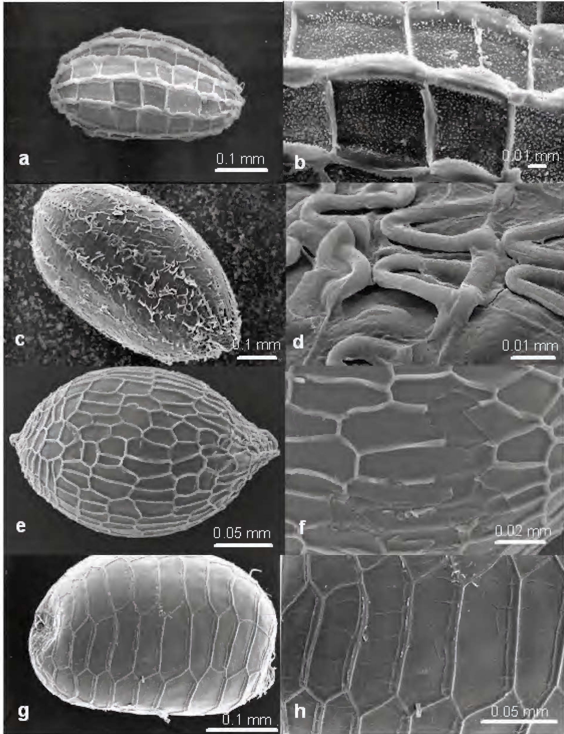
Fig. 10. Seed and seed surface: Eriocaulon truncatum a, b; E. willdenovianum c, d; E. wolseleyi e, f; E. zollingerianum g, h. Material used: a-b from Blake 23348; c-d from Leach 1529; e-f from Lovatt R215; g-h from Clarkson 4409.
